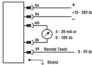
Quick-Disconnect Model (5-pin Mini-Style)
