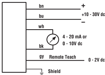
Integral Cable Model
